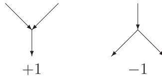
Fig.3. Y-orientations and signs of vertexes.
