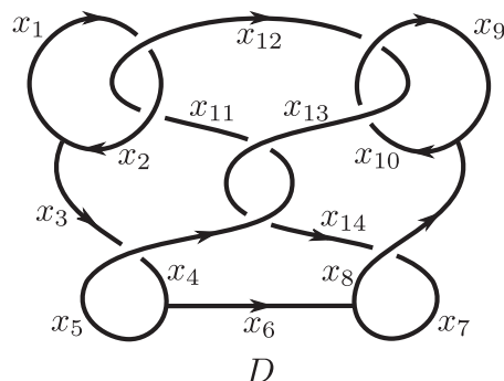
Fig.5. A Y-oriented diagram of a handlebody-knot.
