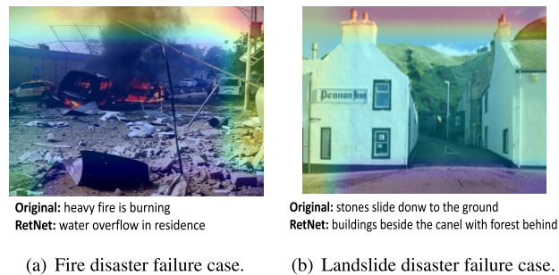
FIGURE 8. Heat map attention of caption from original image and RetNet image in failure case.
