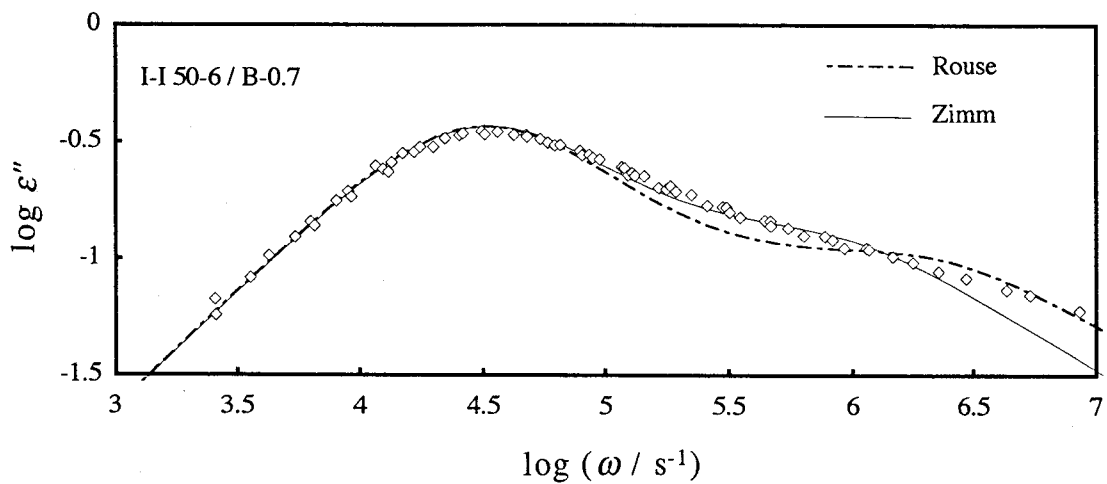
Figure VI-10. Comparison between the Rouse and Zimm models for the shape of \epsilon'' curve of I-I 50-6 in PB-0.7.
