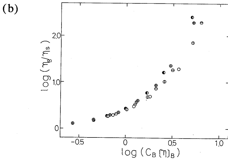
Figure V-20. (a) Double-logarithmic plots of relative viscosity \eta_B/\eta_s vs. PB concentration C_B for PB/heptane solutions at 295K. (b) Same data plotted against C_B[\eta]_B .
