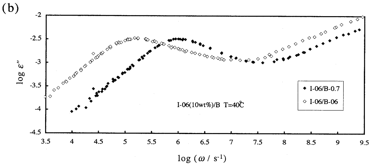
Figure V-31. Master curves of \epsilon'' for blends of (a) PI-49(5wt%)/PB and (b) PI-6(10wt%)/PB at 40°C.
