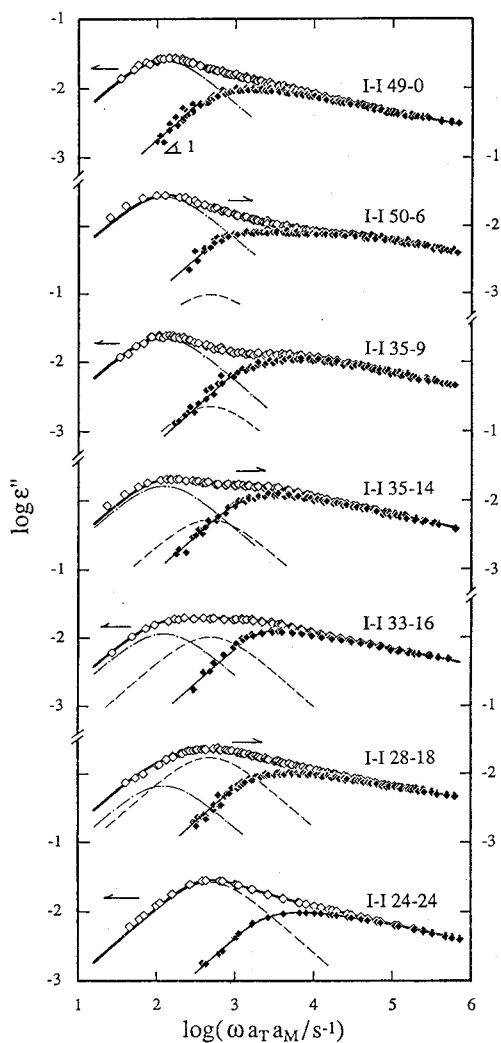
Figure VI-5. Results of the mode-decomposition of the \epsilon'' data (unfilled symbols) for the dipole-inverted PI chains at 40^\circ\text{C} . Linear-least-square-fit with eq VI-16 was made for the decomposition. The dash-dot and dashed curves indicate the contributions from the first and second eigenmodes g_1 D_1(\omega) and g_2 D_2(\omega) , respectively. ( D_p(\omega) = \omega \tau_p / (1 + \omega^2 \tau_p^2) .) The contributions from all higher p -th eigenmodes with p \geq 3 , \epsilon_{p \geq 3}''(\omega) , is shown with the filled symbols. The thick solid curves indicate the re-calculated \epsilon'' = g_1 D_1 + g_2 D_2 + \epsilon_{p \geq 3}'' , with \epsilon_{p \geq 3}'' being evaluated for the thin solid curves that smoothly connect the filled symbols.
