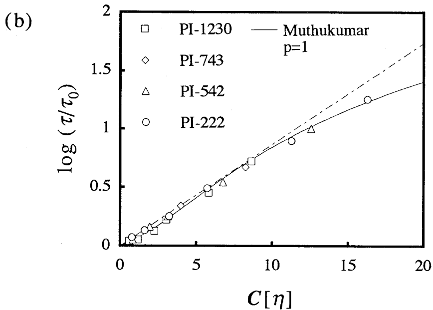
Figure V-12. Comparison with the Muthukumar and Freed theory for C[\eta] dependence of \tau/\tau_0 . (a) Heptane and (b) Cyclohexane solution.
