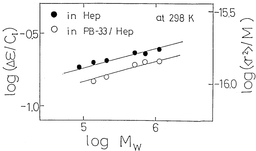
Figure IV-17. Dependence of \Delta\epsilon/C on molecular weight of PI in heptane dilute solution and PB-33/heptane semidilute solution ( C_B = 4.84 \times 10^{-2} \text{ gcm}^{-3} ).
