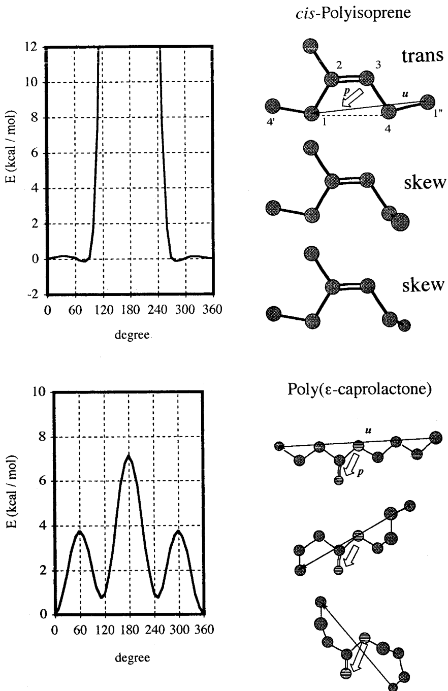
Figure IV-3. Monomer conformation and rotational potential energy for PI and PCL.
