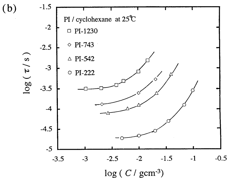
Figure V-8. Concentration dependence of normal mode relaxation time \tau in (a) heptane and (b) in cyclohexane solutions of PI with different M_w .
