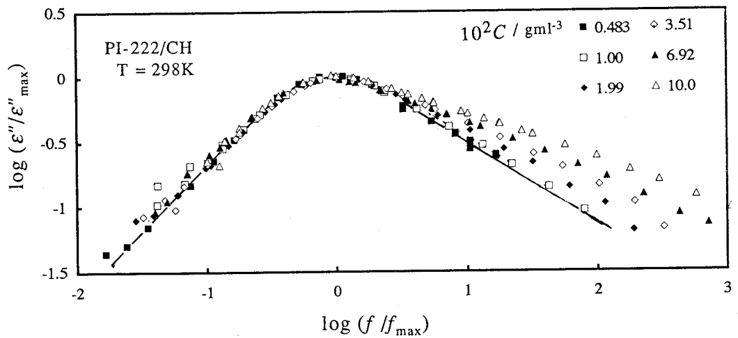
Figure V-15. Reduced \epsilon'' curves for (a) PI-743/heptane and (b) PI-222/cyclohexane solutions of various concentrations. The solid line indicate the predicted curves by Zimm theory.
