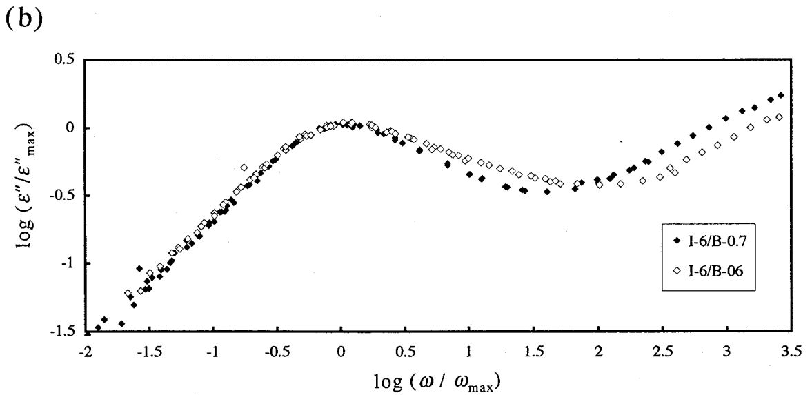
Figure V-33. Comparison of the shapes of \epsilon'' curves for blends of (a) PI-49(5wt%)/PB and (b) PI-6(10wt%)/PB.
