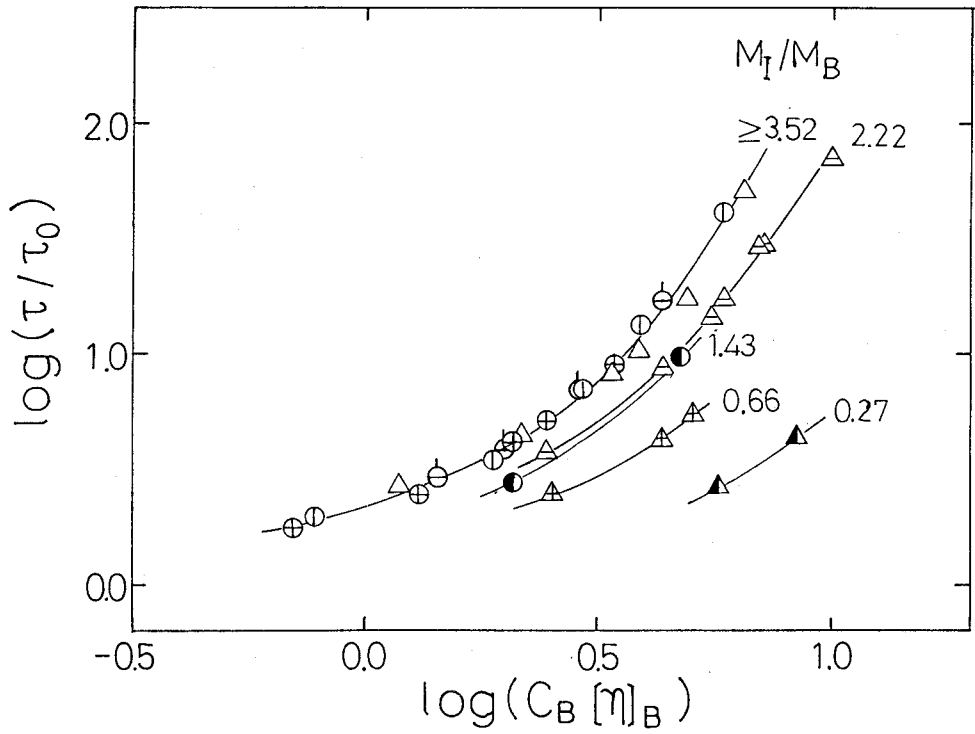
Figure V-21. Double-logarithmic plots of \tau/\tau_0 vs. C_B[\eta]_B . The ratio M_I/M_B is indicated in the curve. The symbols are the same as in Figure V-19.
