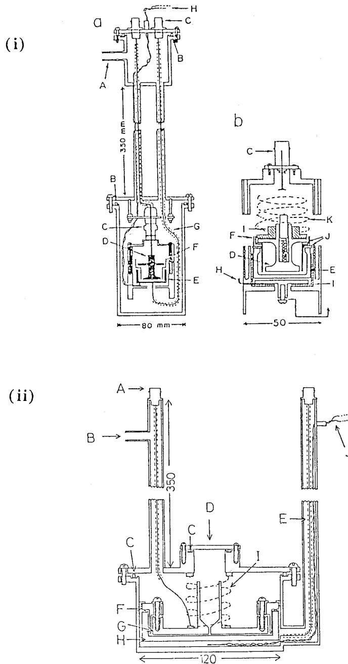
Figure III-3. Sketches of the capacitance cell: (i) standard cell, (ii) large cell.
