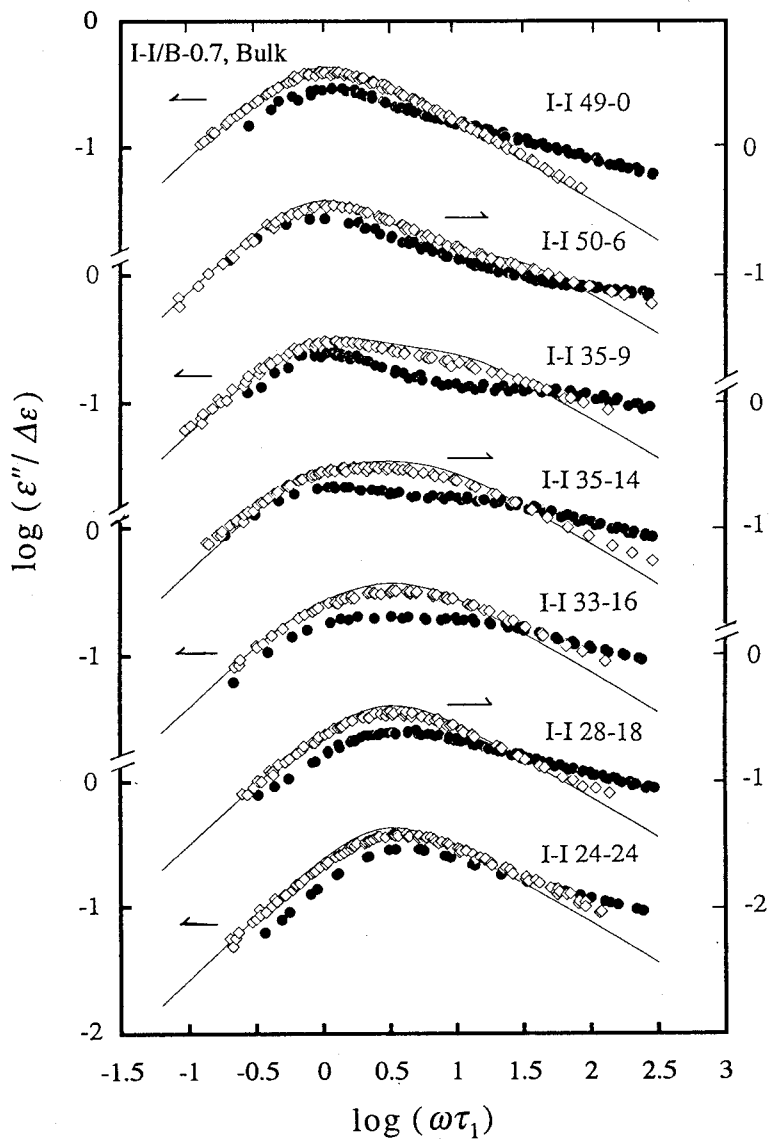
Figure VI-8 Reduced frequency ( \omega\tau_1 ) dependence of the dielectric loss factors \epsilon'' reduced by the relaxation strengths at 40^\circ\text{C} for I-I (5wt%)/PB-0.7 systems (unfilled symbols). The solid circles represent the data of the bulk systems and the solid lines indicate the predicted curves from Zimm model.
