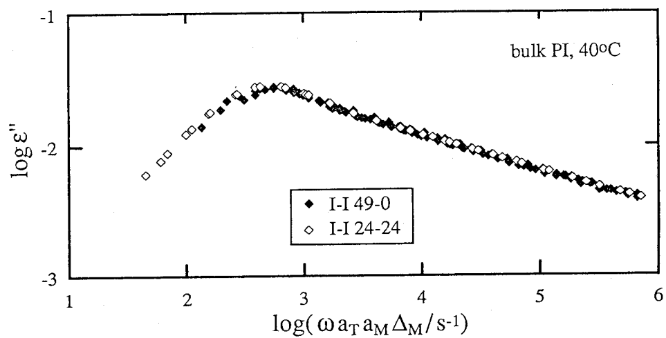
Figure VI-4 Comparison of the \epsilon'' curves at 40^\circ\text{C} for the I-I 49-0 and I-I 24-24 chains. The curve for the former is shifted along the \omega -axis first by a factor a_M = (48.8 / 47.7)^{3.5} = 1.083 (a correction for difference of \tau_1 ) and further by a factor \Delta_M = 3.9 .
