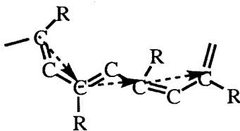
polyacetylene
